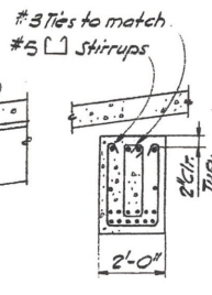
Section e-e
