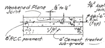
TYPICAL TRANSVERSE WEAKENED PLANE JOINT SECTION A-S10 Scale: 3/4" = 1'-0"
