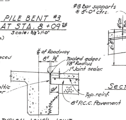
TYPICAL LONG JOINT SECTION C-S10 Scale: 3/4" = 1'-0"
