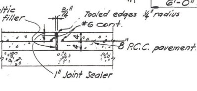
TYPICAL EXPANSION JOINT SECTION B-S10 Scale: 3/4" = 1'-0" Located at Bent #7, #14 & #20 Only
