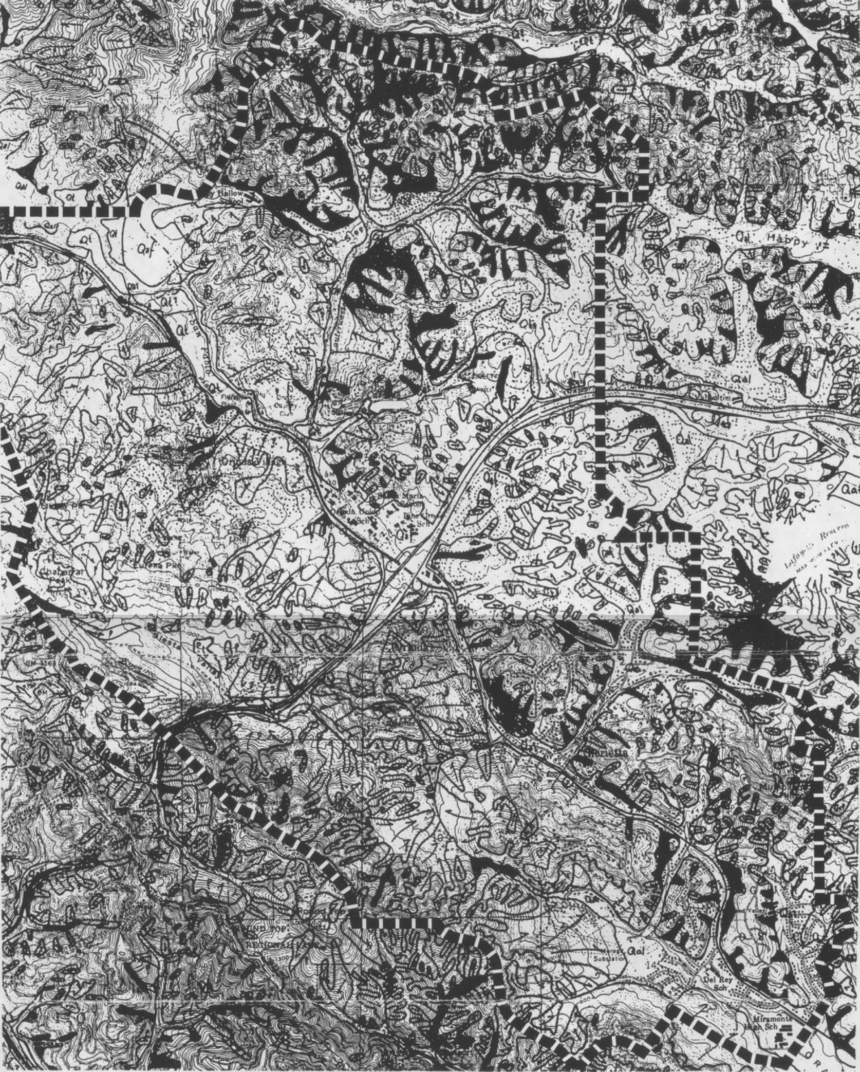
Figure 7: LANDSLIDE AND OTHER SURFICIAL DEPOSITS
