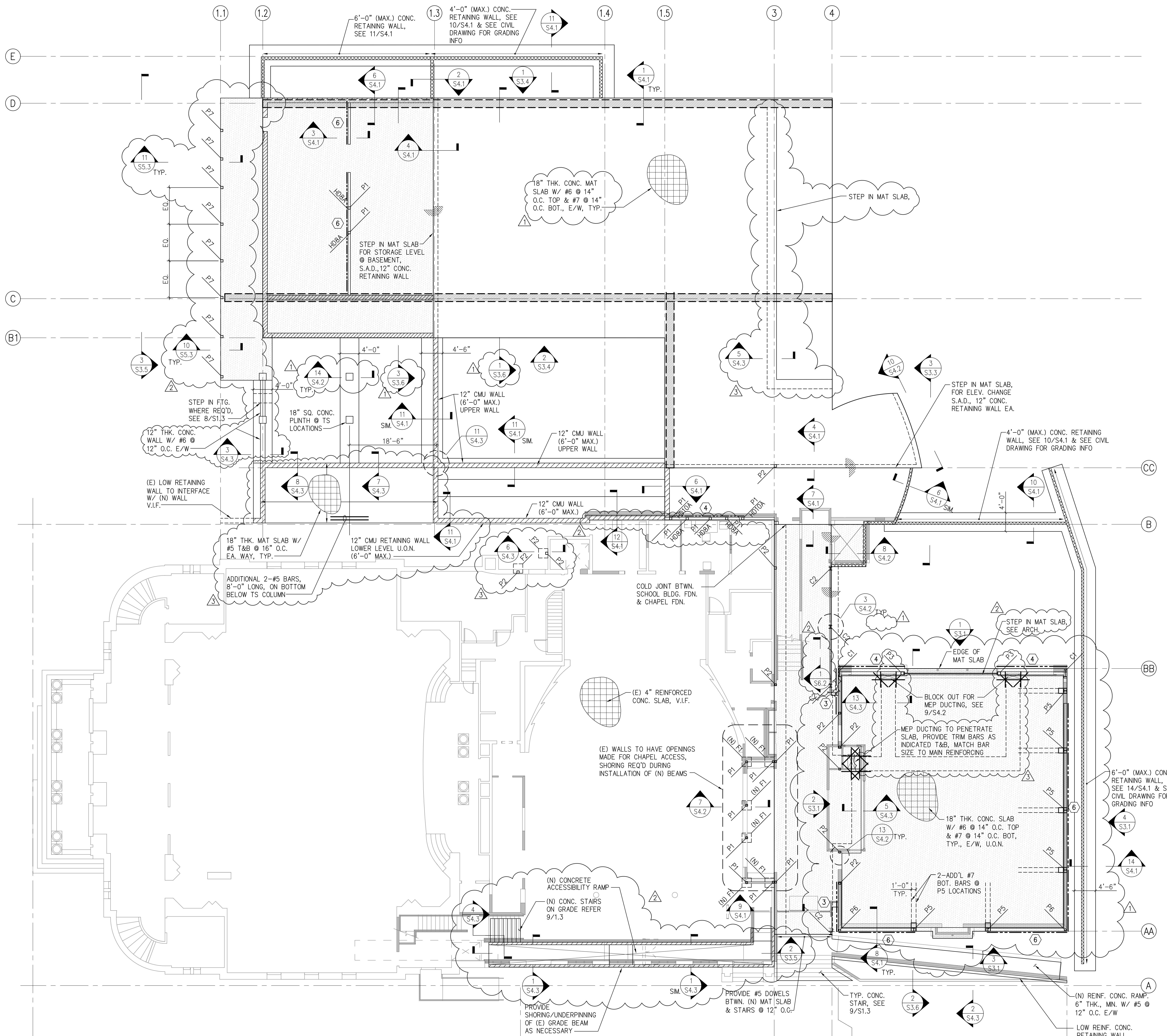
FOUNDATION PLAN
