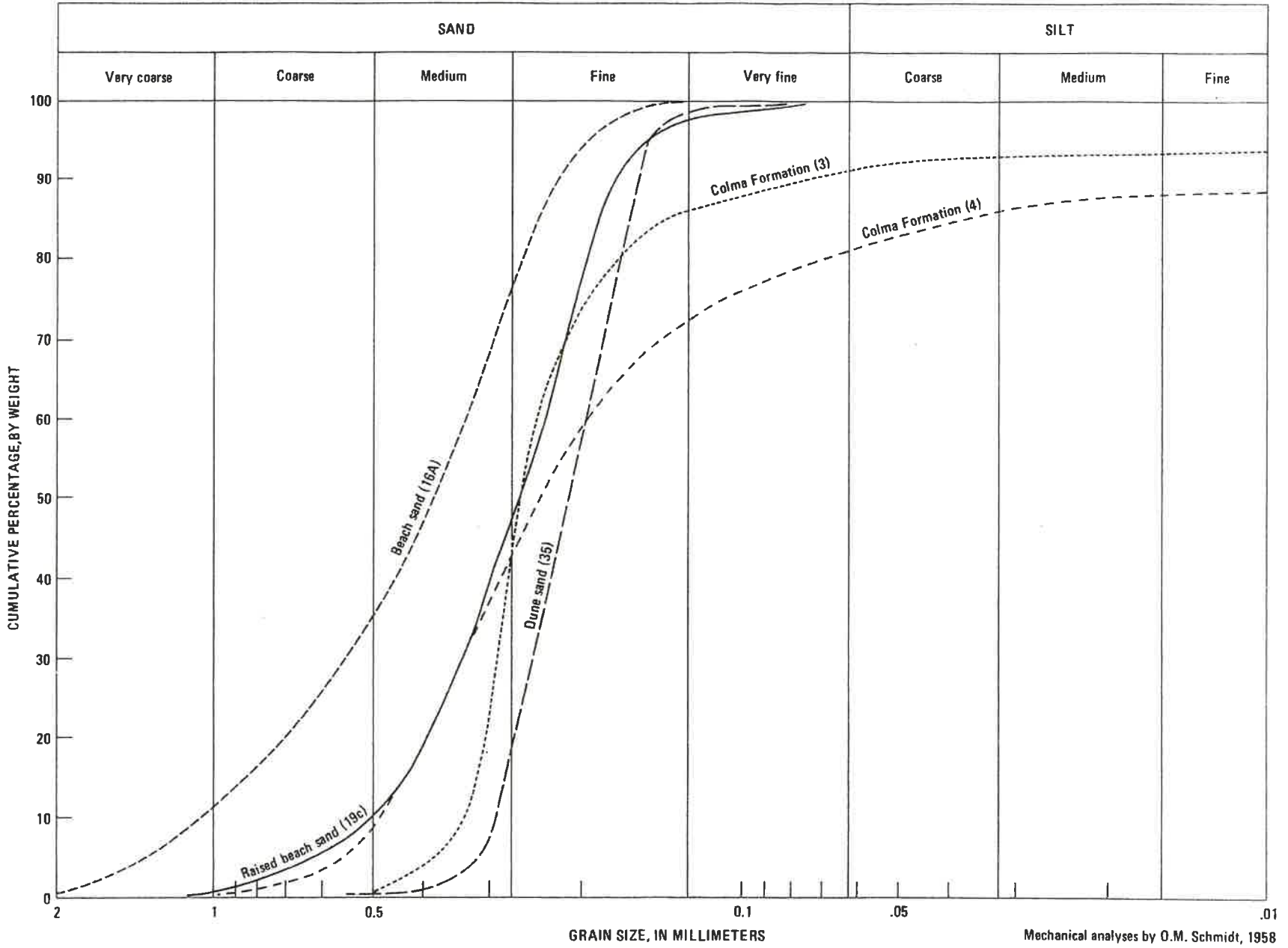
REPRESENTATIVE CUMULATIVE CURVES OF GRAIN SIZES
